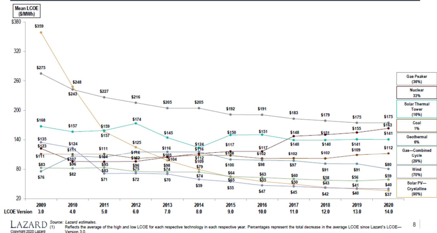
Selected Historical Mean Unsubsidized LCOE Values (1)
